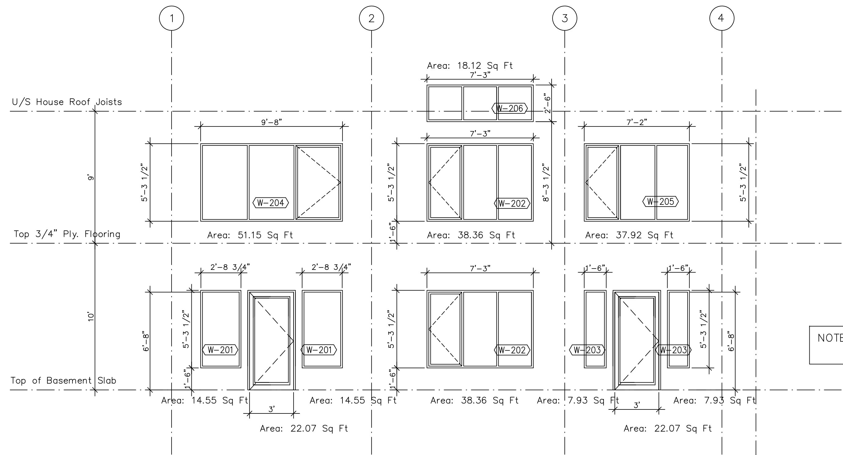
1 FRONT [WEST] ELEVATION A-06 LOT 2 PARTRIDGE DRIVE 1/4" = 1'-0"
