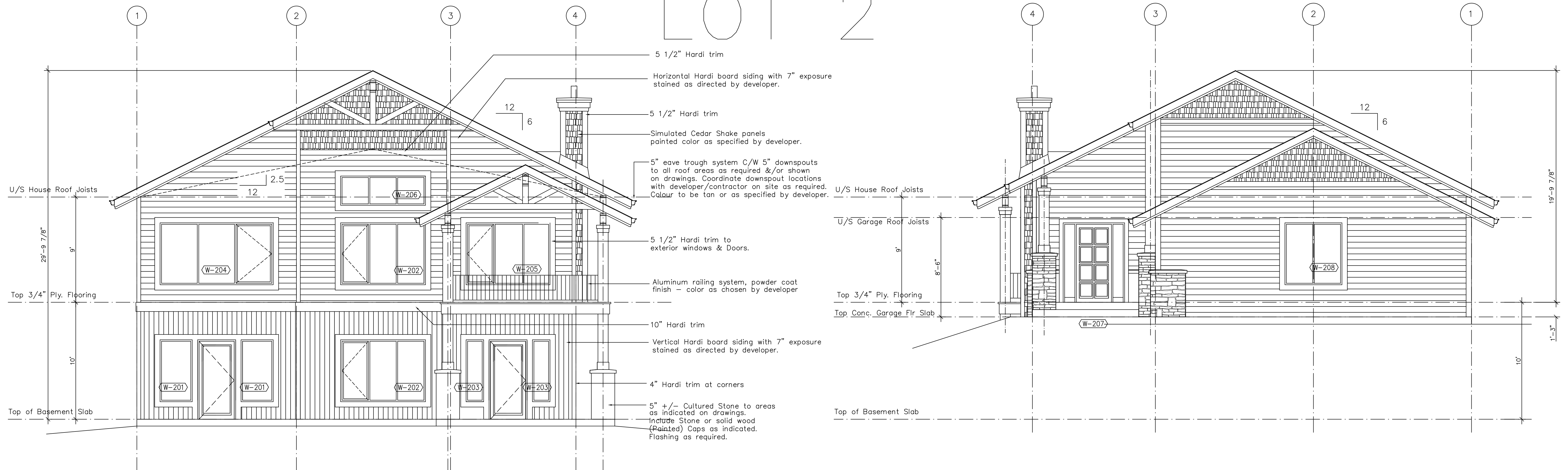
1 FRONT [WEST] ELEVATION A-06 LOT 2 PARTRIDGE DRIVE 1/4" = 1'-0"
